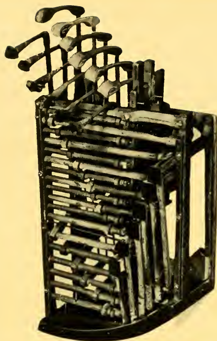
Hammermechanik zu No. 628.
